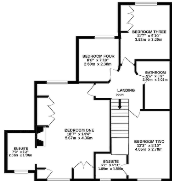
1ST FLOOR 726 sq.ft. (67.5 sq.m.) approx.
